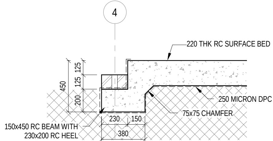
SECTION SC1 - TYPICAL DOOR THRESHOLD 1:20
