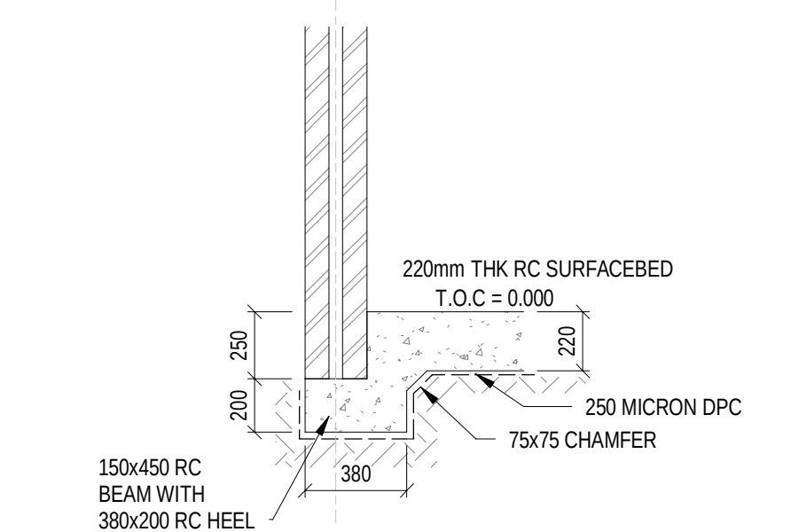
DETAIL 1 - TYPICAL EDGE GROUND BEAM DETAIL 1:25
