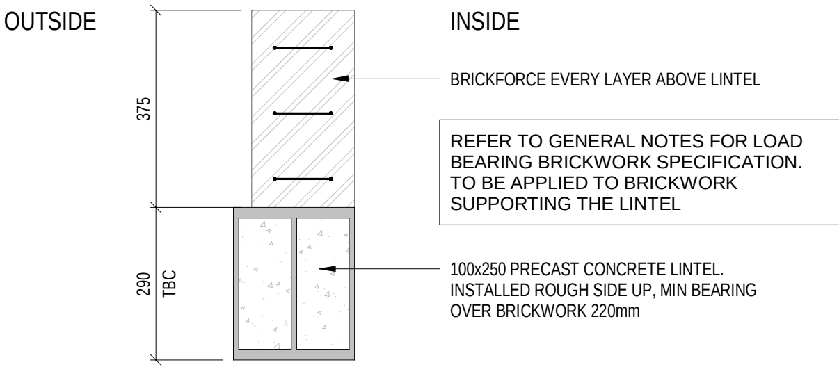
TYPICAL BRICKWORK SUPPORT DETAIL FOR OPENINGS GREATER THAN 3m 1:10
