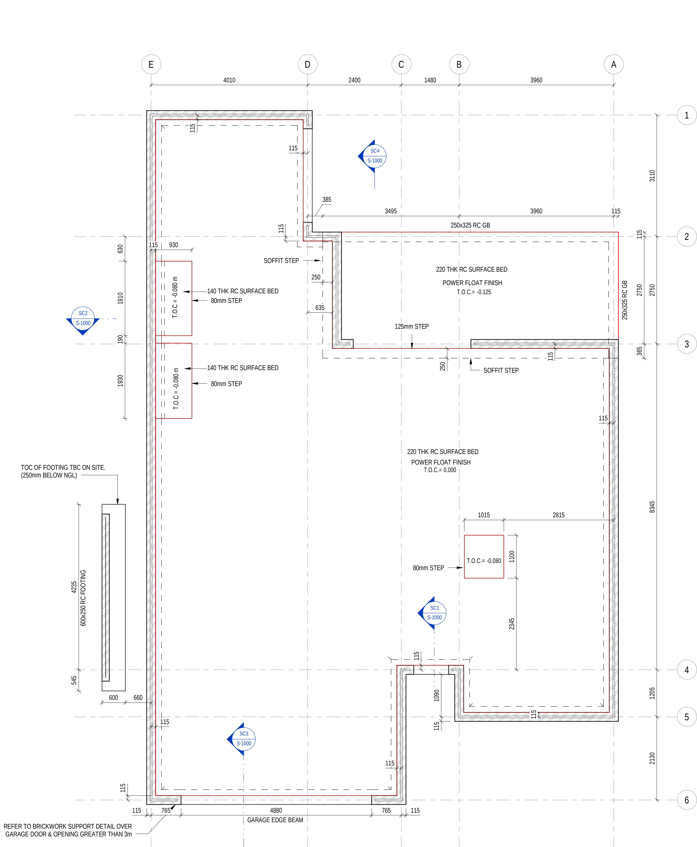
GROUND FLOOR LAYOUT 1:50
