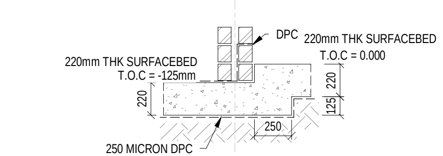
DETAIL 2 - TYPICAL PATIO THRESHOLD DETAIL 1:25
