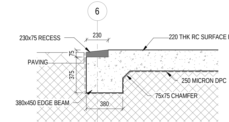
SECTION SC3 - TYPICAL GARAGE THRESHOLD 1:20
