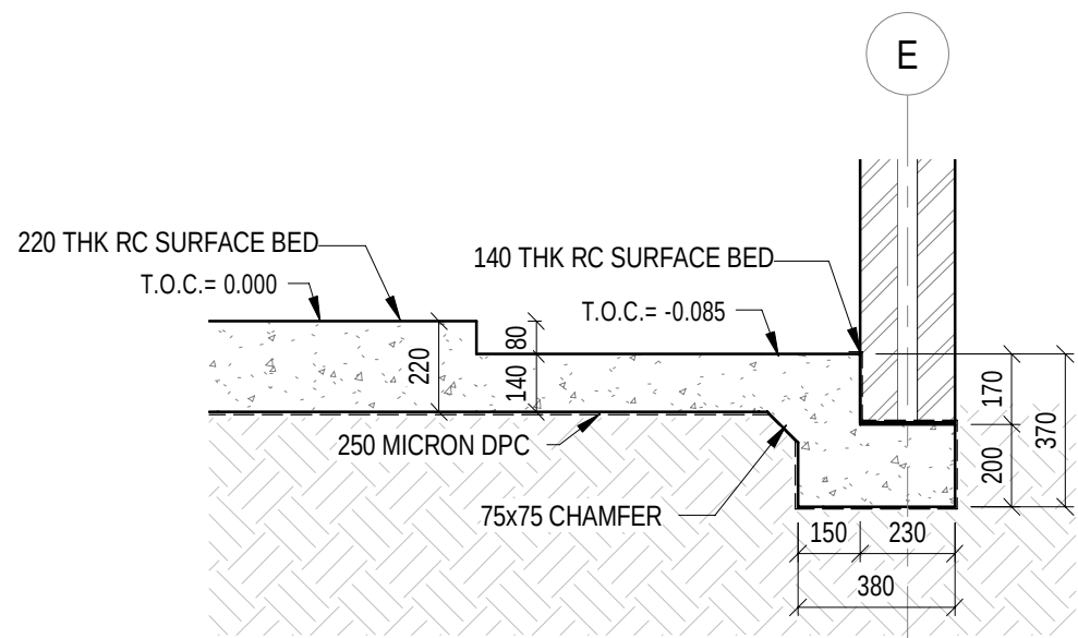
SECTION SC2 - TYPICAL SHOWER RECESS DETAIL 1:20
